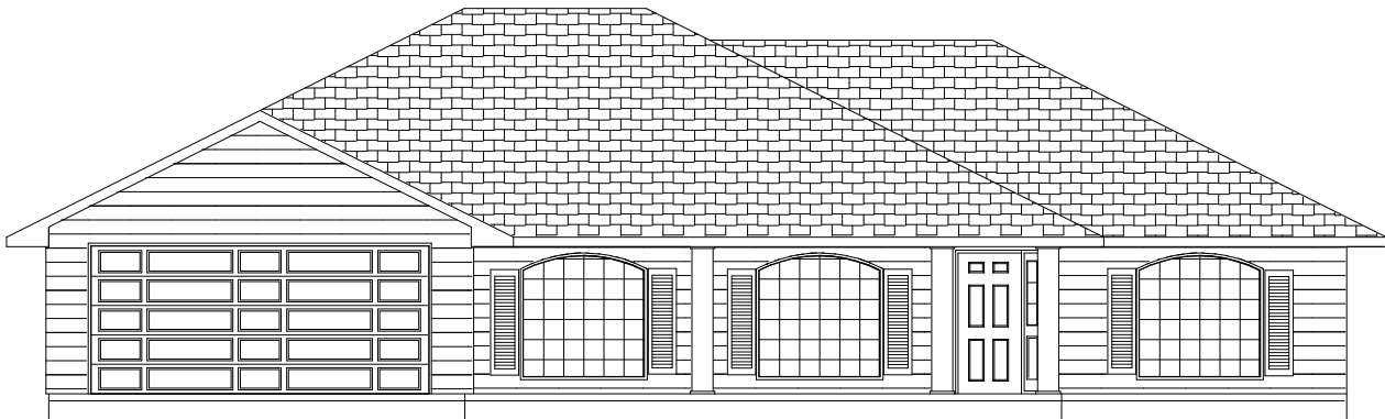
UPGRADE ELEVATION
